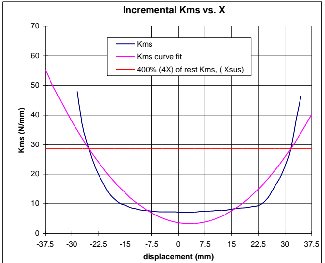
manual Kms fit -28.5 mm to 34.5 mm
