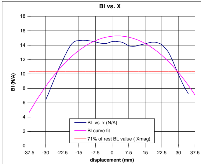
manual BL fit -30 mm to 34.5 mm
